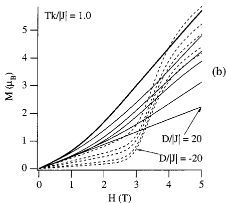
Figure 16. (a) Isothermal magnetizations at 2 and 5 K for \text{Fe}_2\text{Cl}_4(2,2'\text{-bpym})_3 . Solid lines are the theoretical behaviors calculated using the anisotropic model results. (b) Influence of the single-ion anisotropy parameter, D , on the isothermal magnetization.
