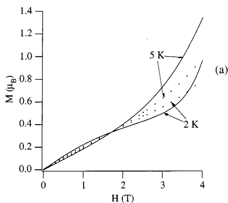
Figure 15. Anisotropic model for an antiferromagnetic dinuclear complex of spins S = 2 showing the influence of the sign and magnitude of the single-ion anisotropy parameter, D .
