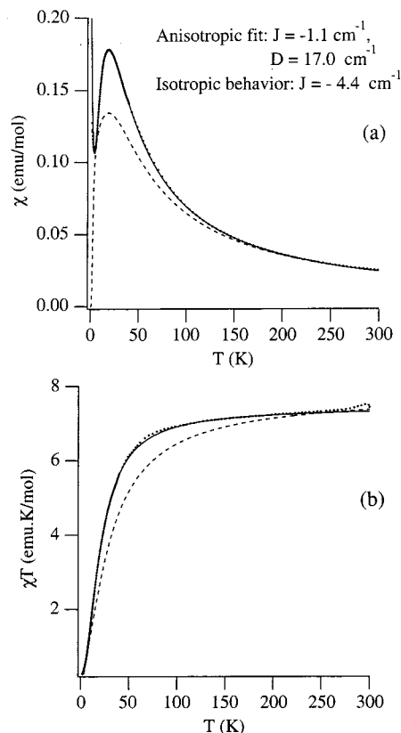
Figure 14. Thermal dependence of the (a) susceptibility and of (b) the product \chi T for Fe_2Cl_4(2,2'-bpy)_3 . Dotted lines are the theoretical behaviors of fully isotropic antiferromagnetic dimers. The best fit to the anisotropic model is shown as a solid line.
