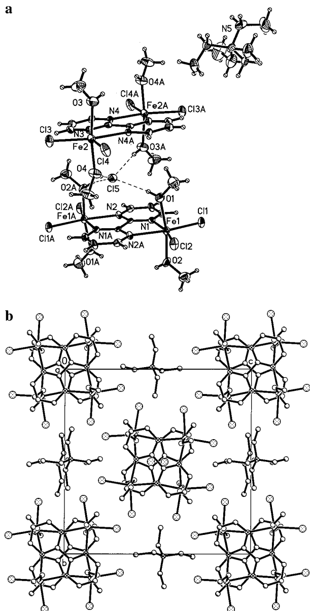
Figure 8. (a) ORTEP representation of [\text{Et}_4\text{N}]\text{Cl}\cdot[\text{Fe}_2\text{Cl}_4(\text{MeOH})_4(\mu\text{-}2,2'\text{-bpy})] ( 9 ) at the 40% probability level and (b) packing diagram.
