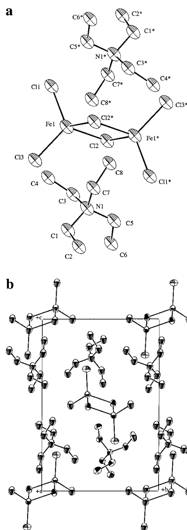
Figure 2. (a) ORTEP representation of [\text{Et}_4\text{N}]_2[\text{Fe}_2\text{Cl}_6] ( 2 ) with thermal ellipsoids at the 50% probability level and (b) packing diagram.
