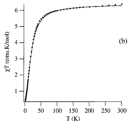
Figure 17. Thermal dependence of the susceptibility (a) and of the product \chi T (b) for [\text{Et}_4\text{N}]\text{Cl} \cdot [\text{Fe}_2\text{Cl}_4(\text{MeOH})_4(\mu\text{-}2,2'\text{-bpym})] .
