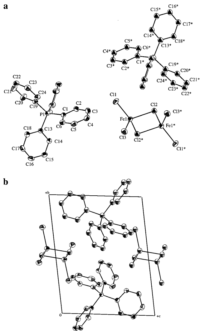
Figure 1. (a) ORTEP representation of [\text{PPh}_4]_2[\text{Fe}_2\text{Cl}_6] ( 1 ) with thermal ellipsoids at the 50% probability level and (b) packing diagram.
